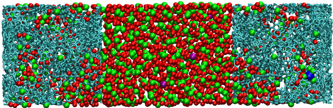
Figure 1: The simulation cell is constituted of two porous electrodes held at constant potential (cyan C atoms). The electrolyte is composed of a \text{FeCl}_3 or \text{FeCl}_2 unit dissolved in EMIM- \text{BF}_4 , modeled using a coarse-grained force-field 32 (red: the three interaction sites of EMIM + , green: the single site of \text{BF}_4^- , blue: Fe (III) cation and violet: \text{Cl}^- anions).
