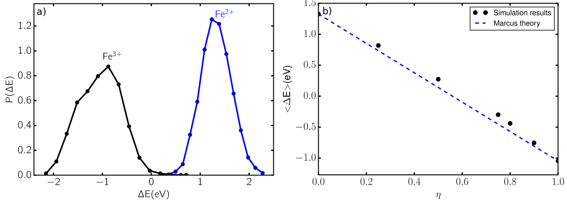
Figure 2: a) Probability distribution of the vertical energy gap in reduced and oxidized states, b) Average vertical energy gap for \text{Fe}^{3+}/\text{Fe}^{2+} in RTILs with various coupling parameters \eta .
